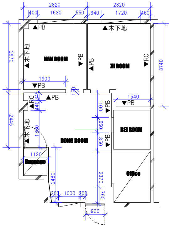
AAA Gallery Whole view SS:1/80
